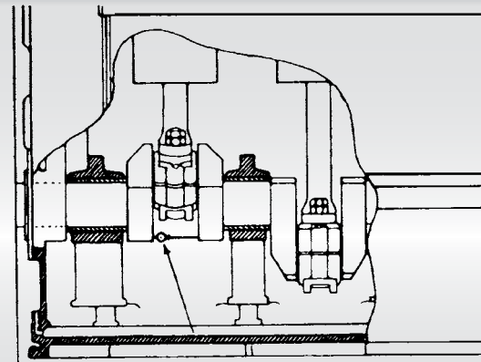
STRAIN GAUGE APPLIED TO CRANK OF DIESEL ENGINE TO DETERMINE IMPROPER ALIGNMENT.
